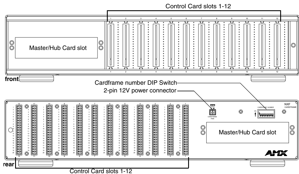
FIG. 1 NXF CardFrame
